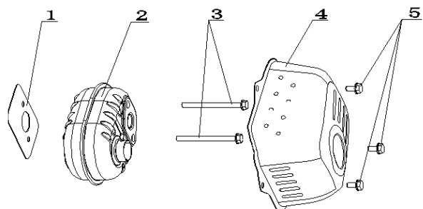
Muffler Ass'y
