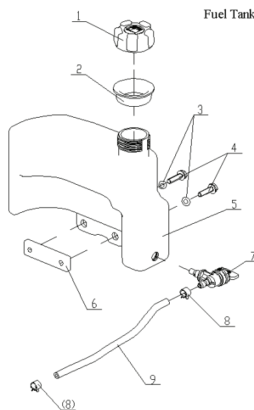
Fuel Tank Ass'y
