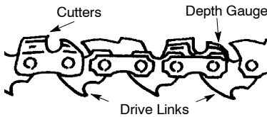
Drive Links
