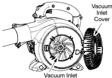
Vacuum Inlet
