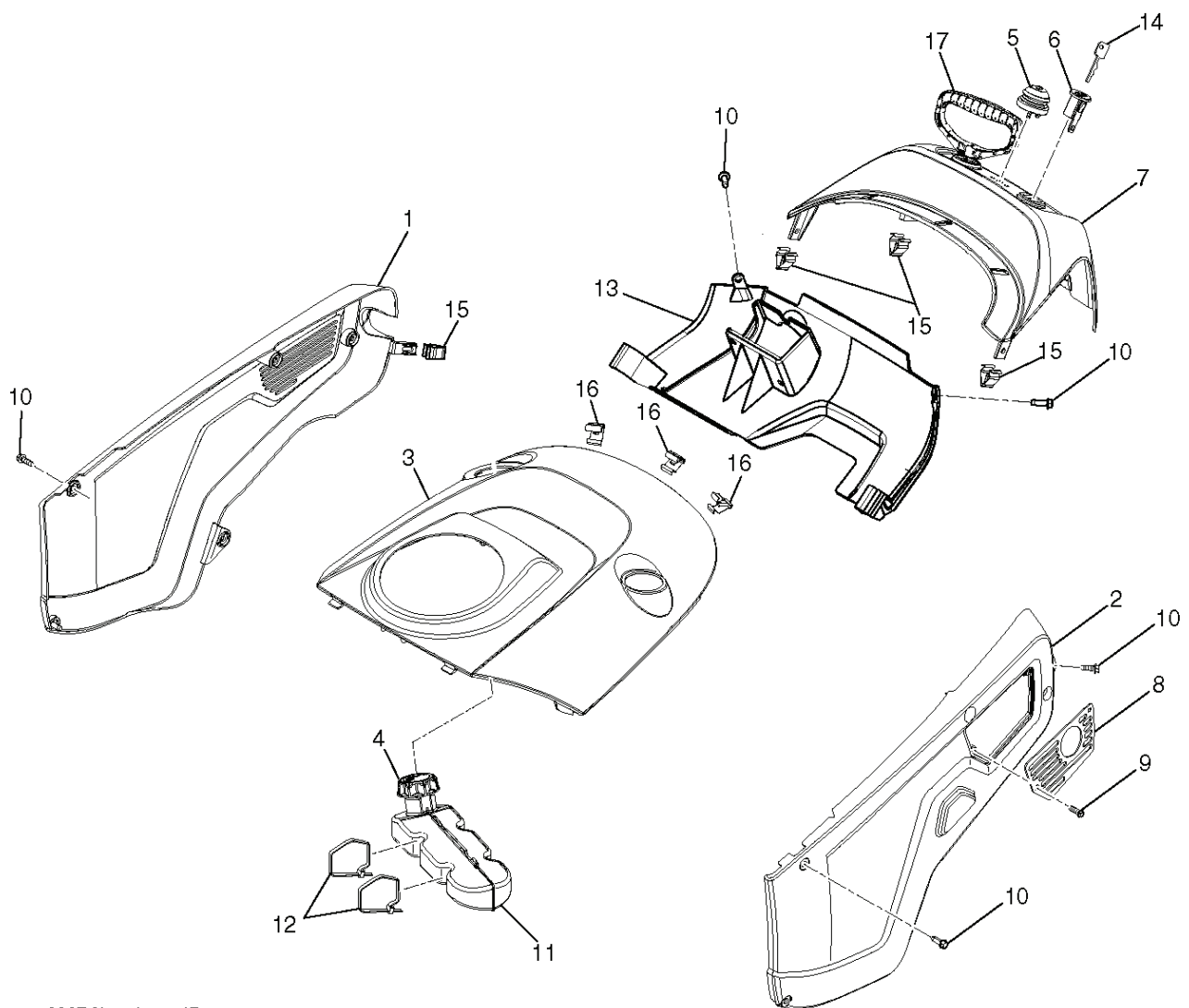
SSST-Shroud asm_17
