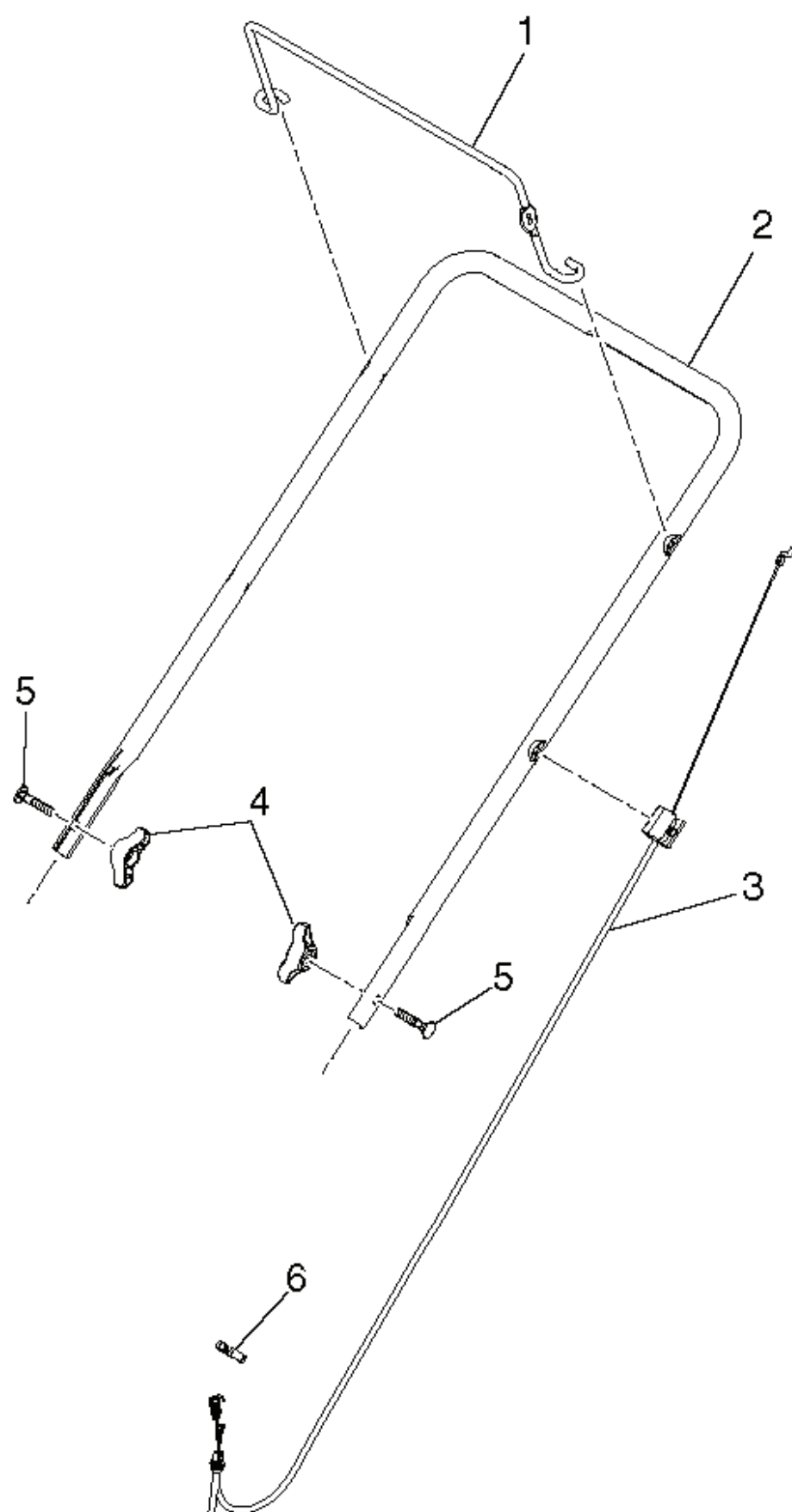
SSST-Handle asm_1
