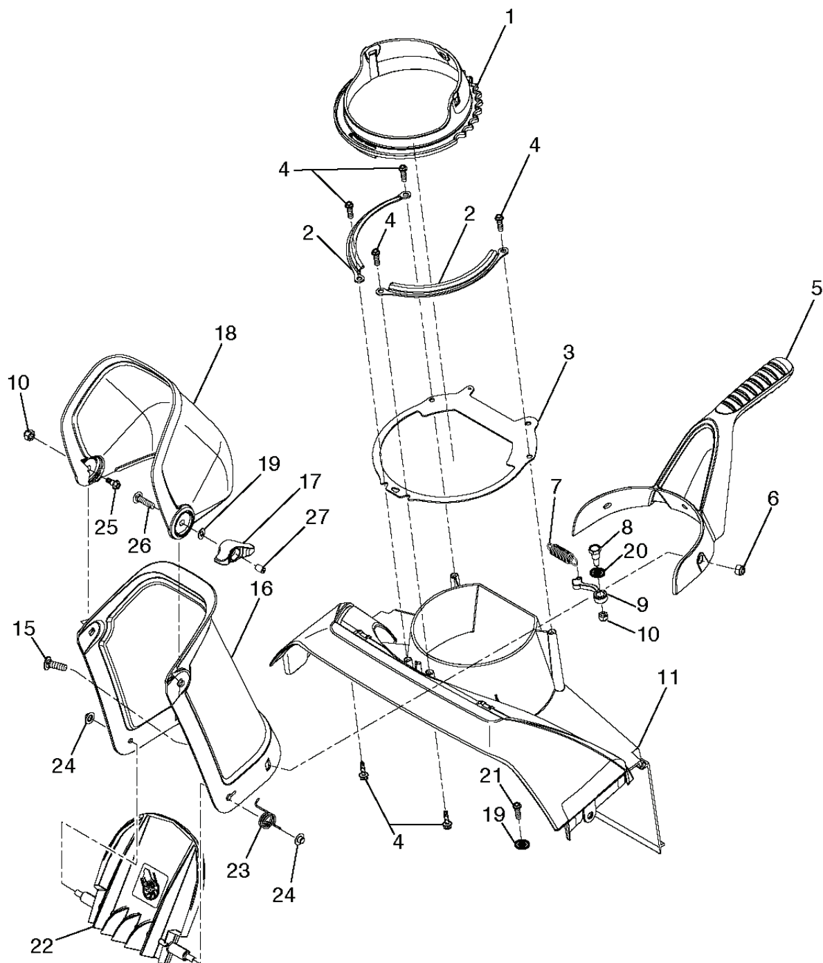
SSST-Chute asm_12
