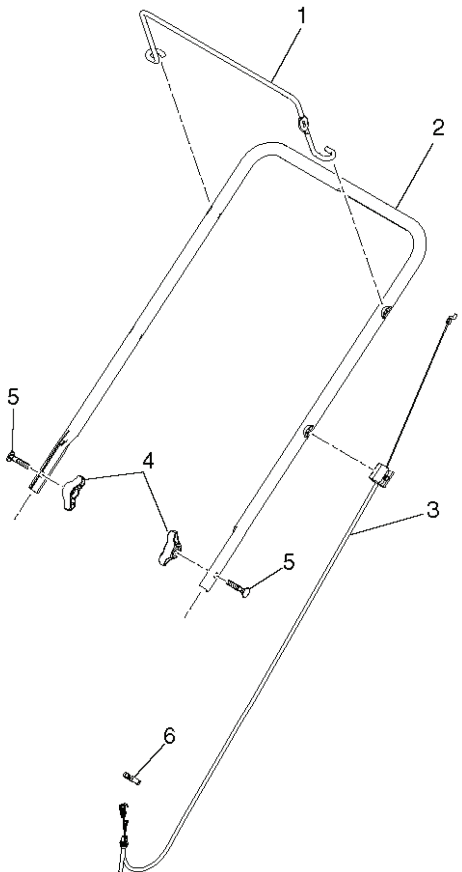
SSST-Handle asm_1
