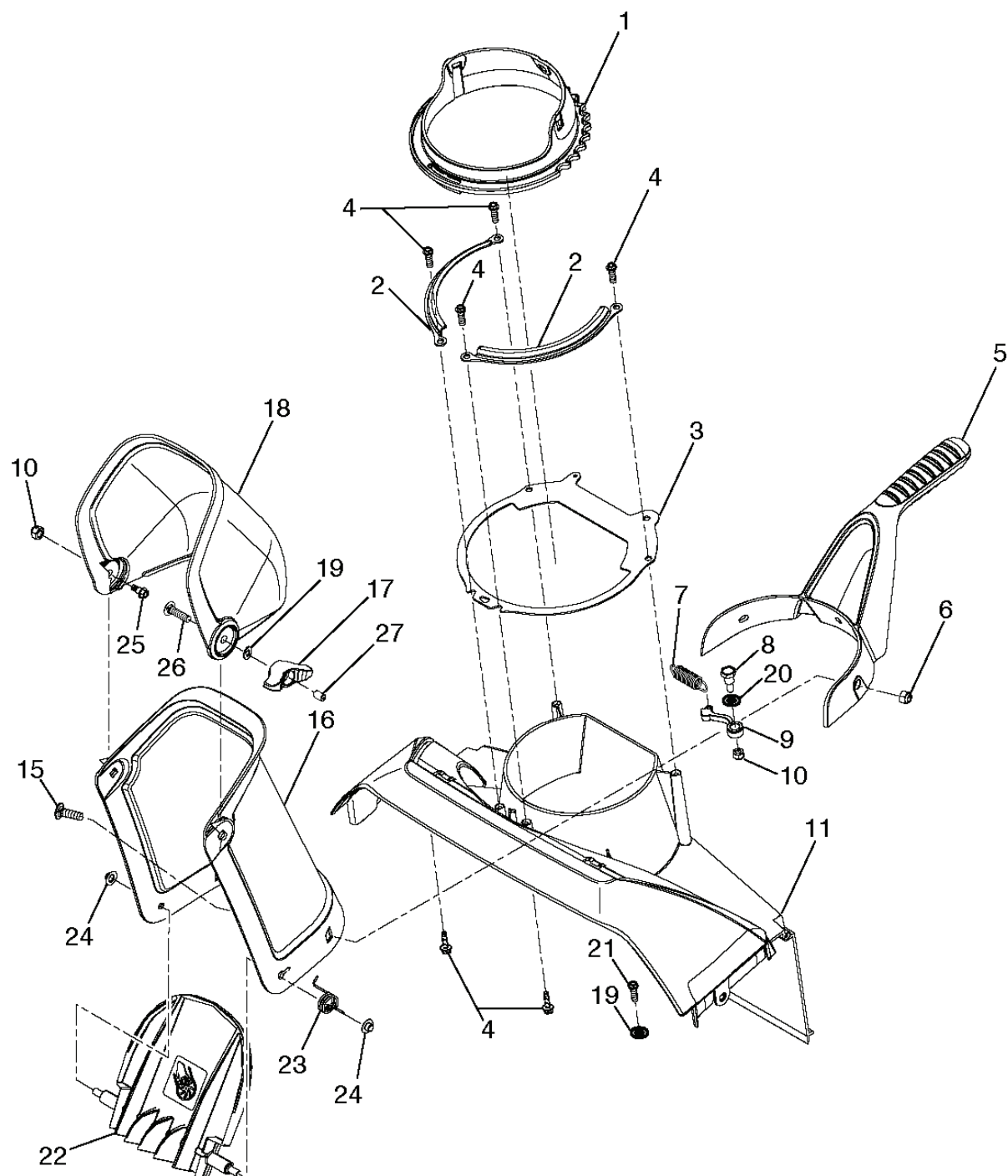
SSST-Chute asm_12
