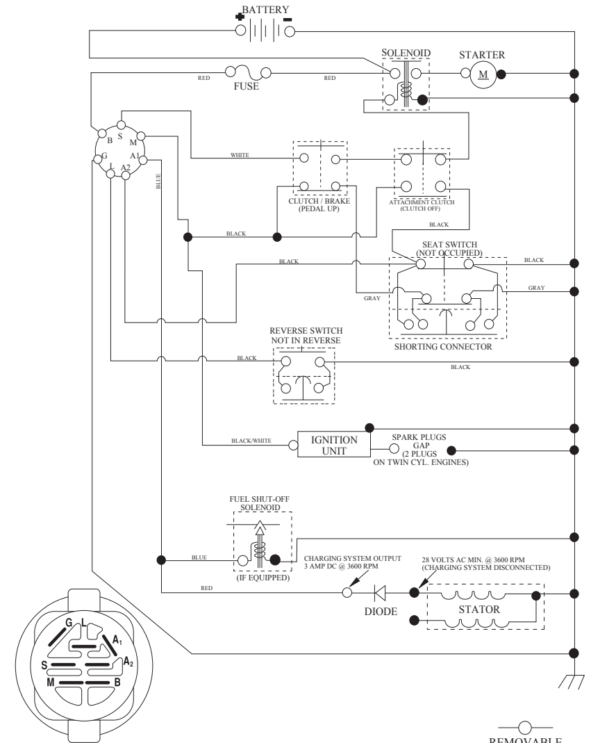
IGNITION SWITCH
